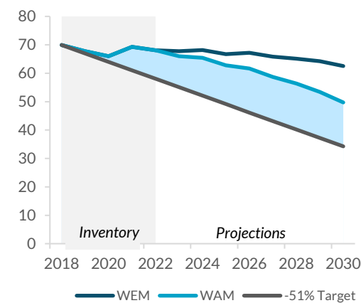
Figure 22 MtCO 2 e
