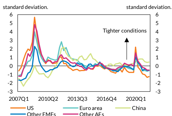
Chart 1: Global financial conditions remain accommodative reaching levels not seen since before the Global Financial Crisis IMF financial conditions index
